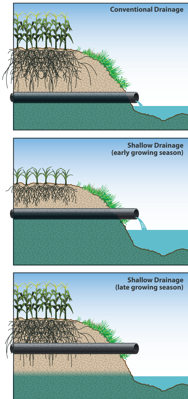
Figure 18: Shallow drain placement removes less excess water than conventional drainage, but still meets crop growth needs.
