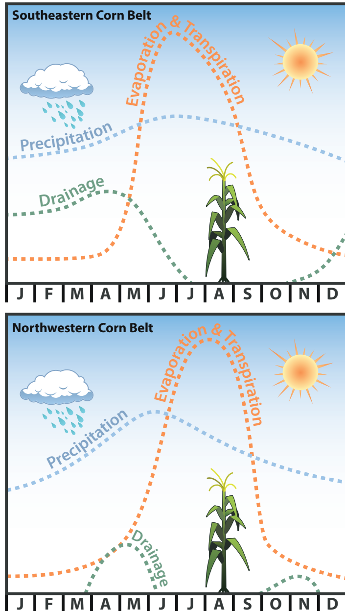
Figure 6: Generic components of the annual water balance for mid-western conditions. Evapotranspiration (orange line) exceeds precipitation (blue line) during the height of the growing season, but at other times, precipitation exceeds evapotranspiration, leading to excess soil water and drain flow (green line). Southeastern examples include Indiana and Ohio, and northwestern examples include North and South Dakota.
